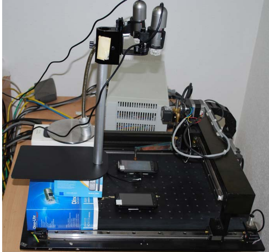
(b) System with multiple mobiles under test
